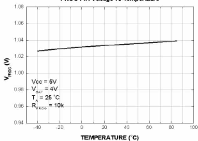
PROG Pin Voltage vs Temperature
