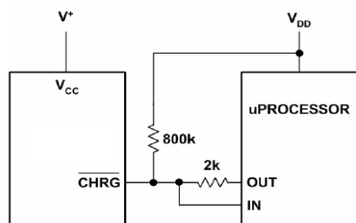
Figure 10. Using a Microprocessor to Determine \overline{\text{CHRG}} State
