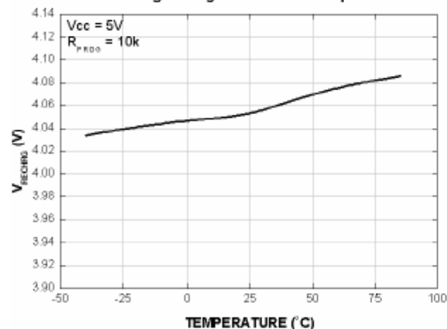
Recharge Voltage Threshold vs Temperature
